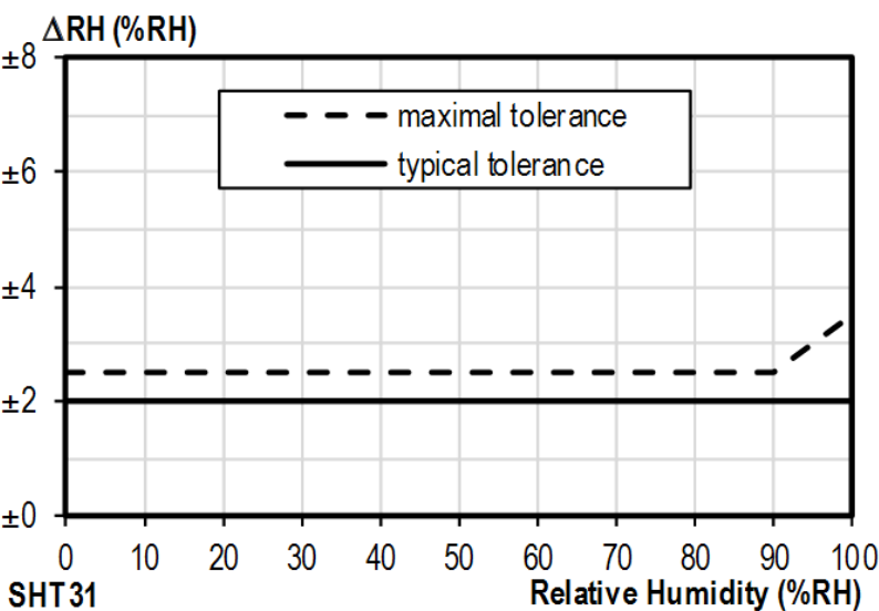
Fig. 16 – Accuracy of humidity measuring
