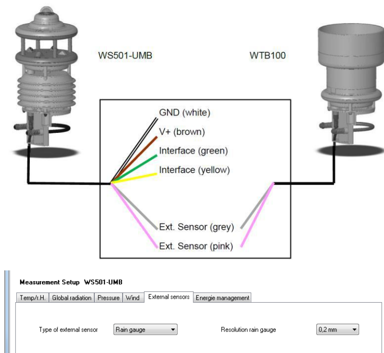
Figure 40: Example WS501-UMB and WTB100
